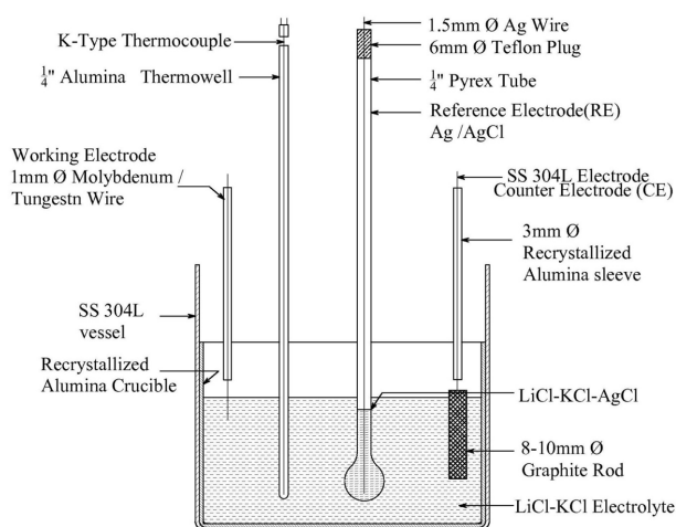
Fig. S2. The schematic of the electrochemical cell assembly.
