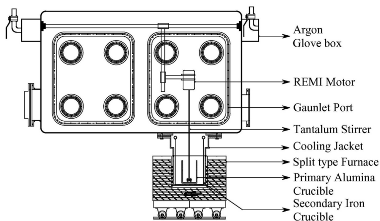
Fig. S1. The schematic diagram of experimental set up for conversion reaction.
