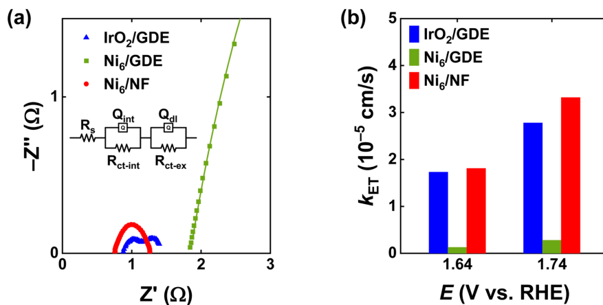
Fig. S10. (a) Nyquist plots at 1.74 V vs. RHE measured on Ni 6 /NF (0.1 mg), Ni 6 /GDE (0.5 mg), and IrO 2 /GDE (4.8 mg). (b) Electron transfer constant ( k_{ET} ) of IrO 2 /GDE, Ni 6 /GDE, and Ni 6 /NF electrodes measured at 1.64 V and 1.74 V vs. RHE in 1.0 M KOH solution.
